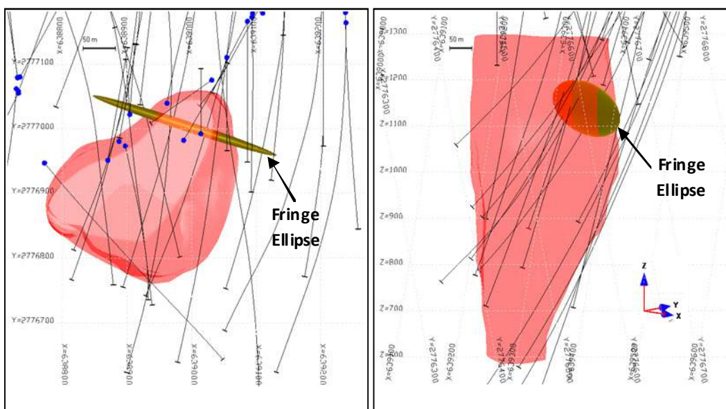
Figure 92: Plan view and 3D view of the Fringe and the N108° ellipsoid.
