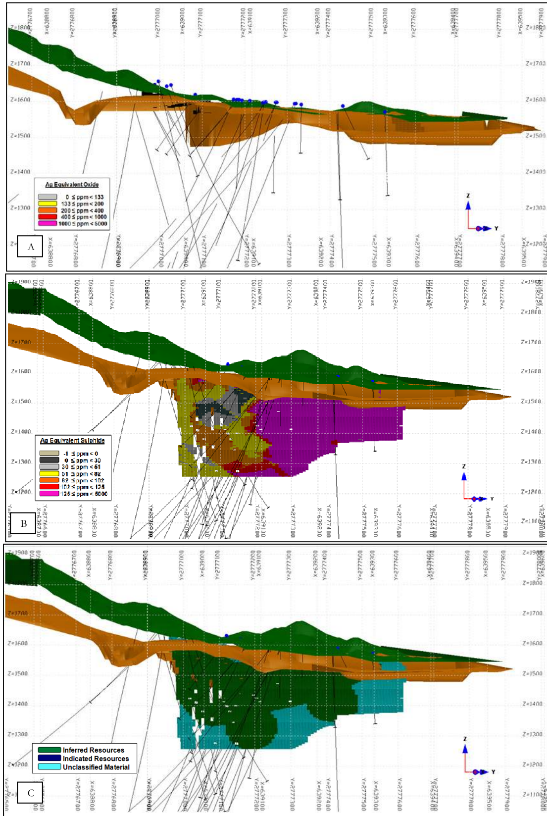
Figure 73: Oxide and sulphide block models, and classification of the El Jal vein, looking N30°.
