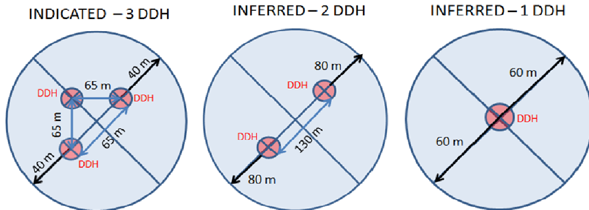
Figure 50: Visual representation of indicated and inferred classifications.
