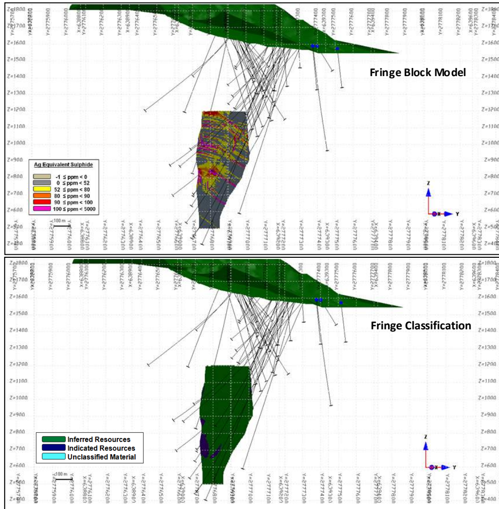
Figure 98: Fringe block model and classification, looking N290°.
